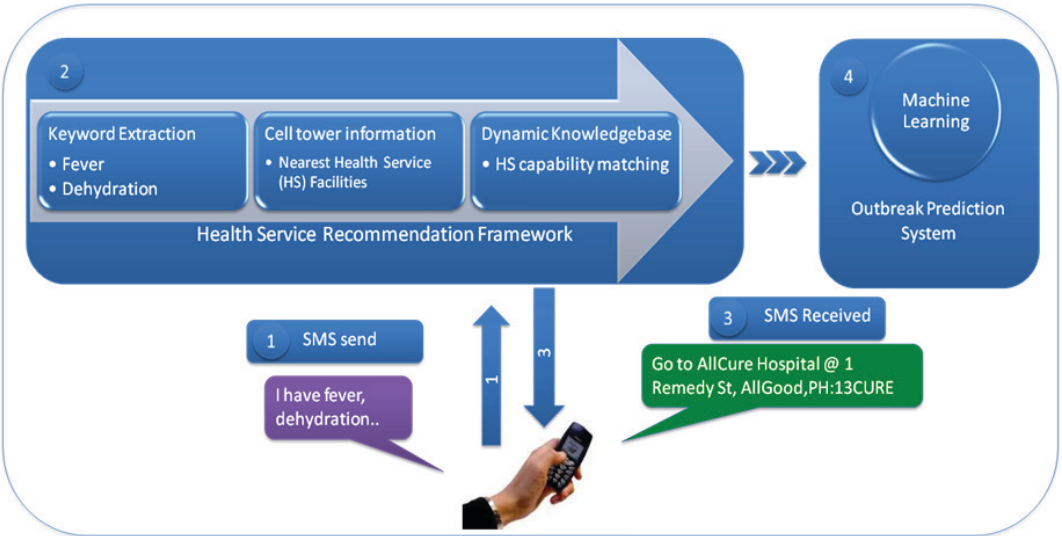
Figure 2. Recommendation Framework.
